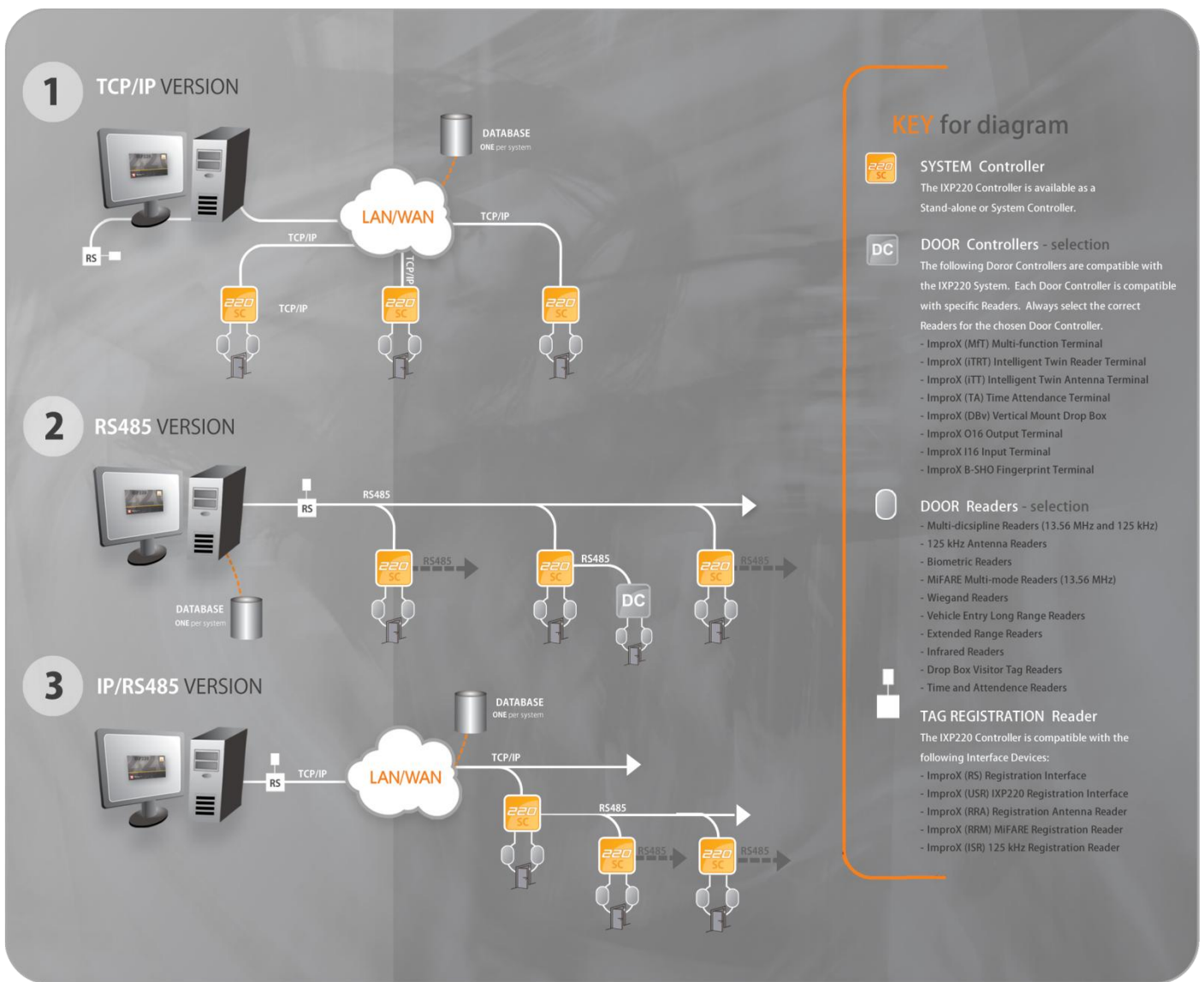
Figure 1: IXP220 System Overview
