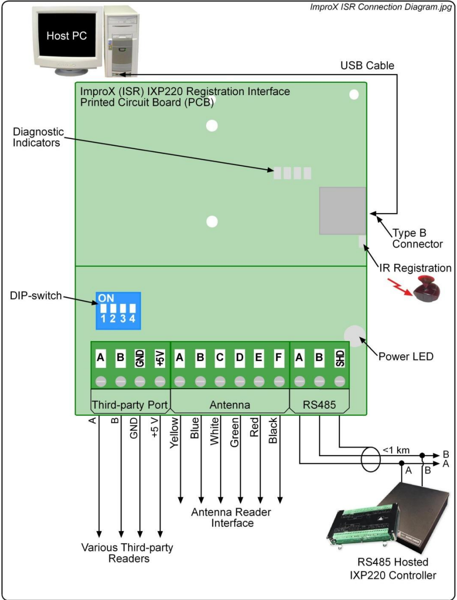
Figure 1: Typical ImproX ISR Electrical Connections
